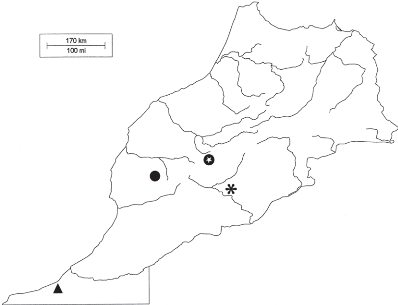
Fig. 8. Type localities of Butheoloides (B.) maroccanus (black circle). B. (B.) occidentalis (black triangle). B. (B.) slimanii sp. n. (black circle with white star) and B. (G.) aymerichi (black flower) in Morocco.
